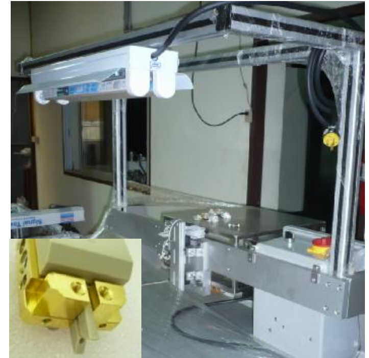
Auto bonding m/c
